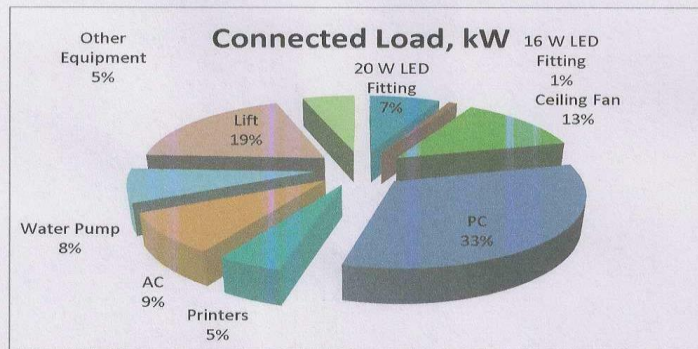
Chart No 1: Details of Connected Load:
